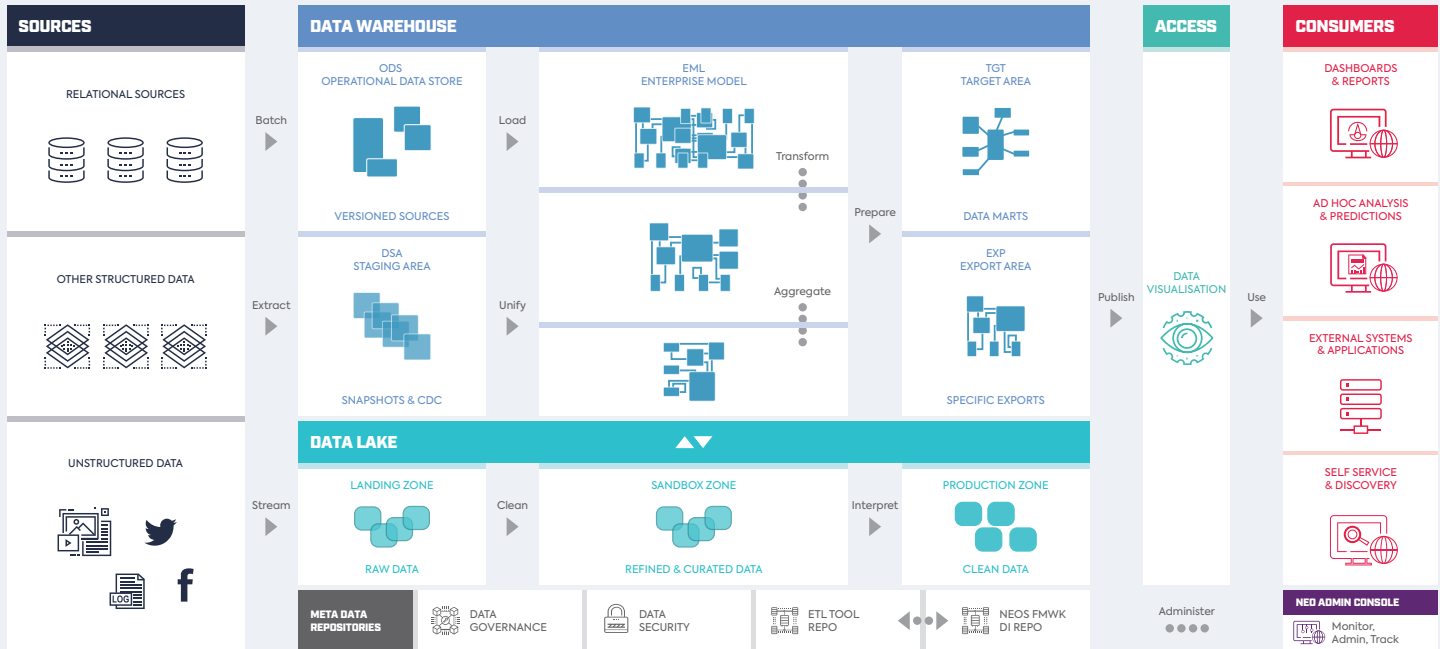
Reference Logical Architecture of Data Analytics Platform used on an array of different projects.
